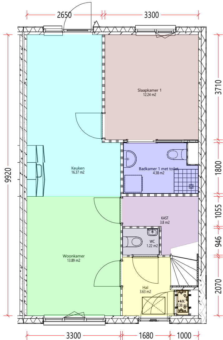
Begane_grond
