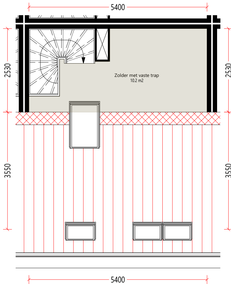
Zolder
