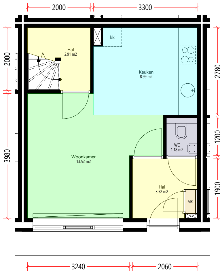
Begane_grond
