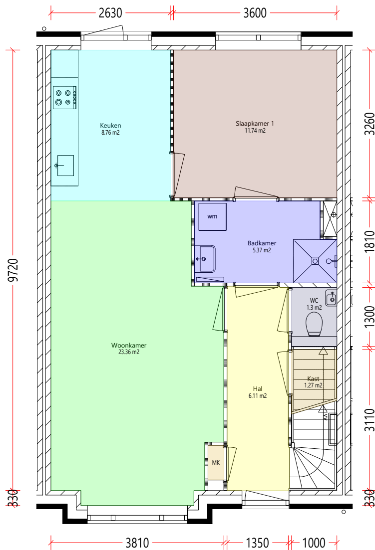
Begane_grond
