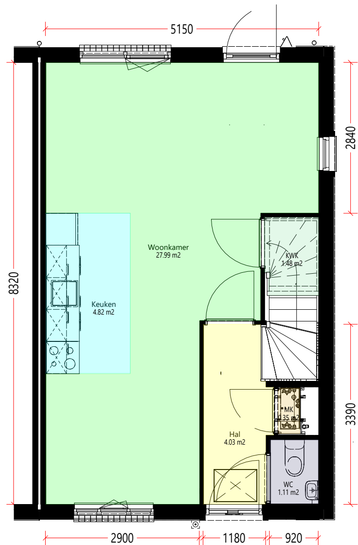
Begane_grond
