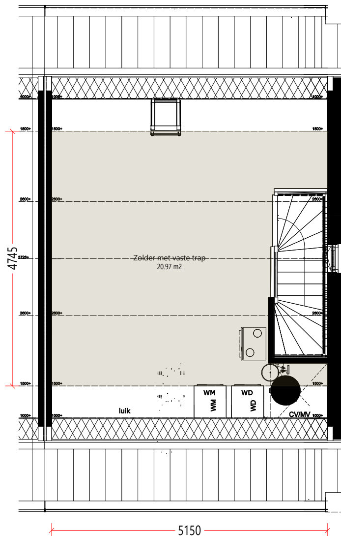
Zolder
