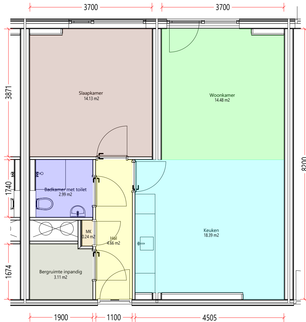
Begane_grond
