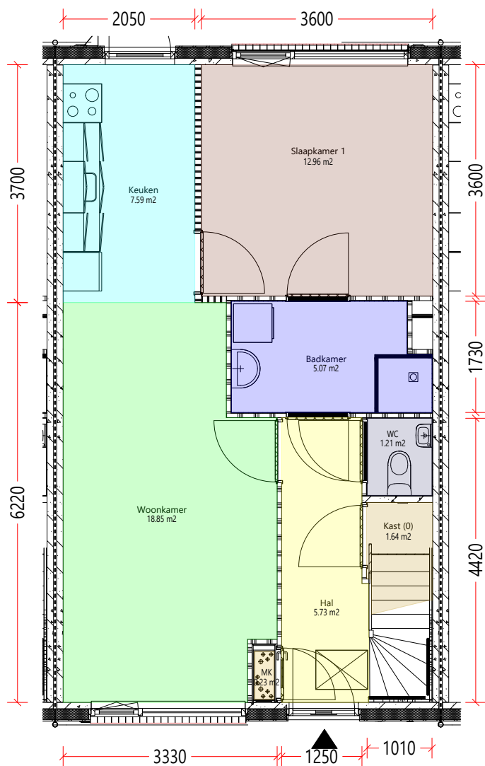
Begane_grond
